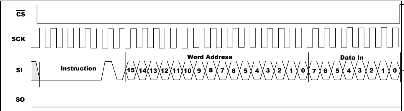
Figure 5-6. WRITE Sequence
