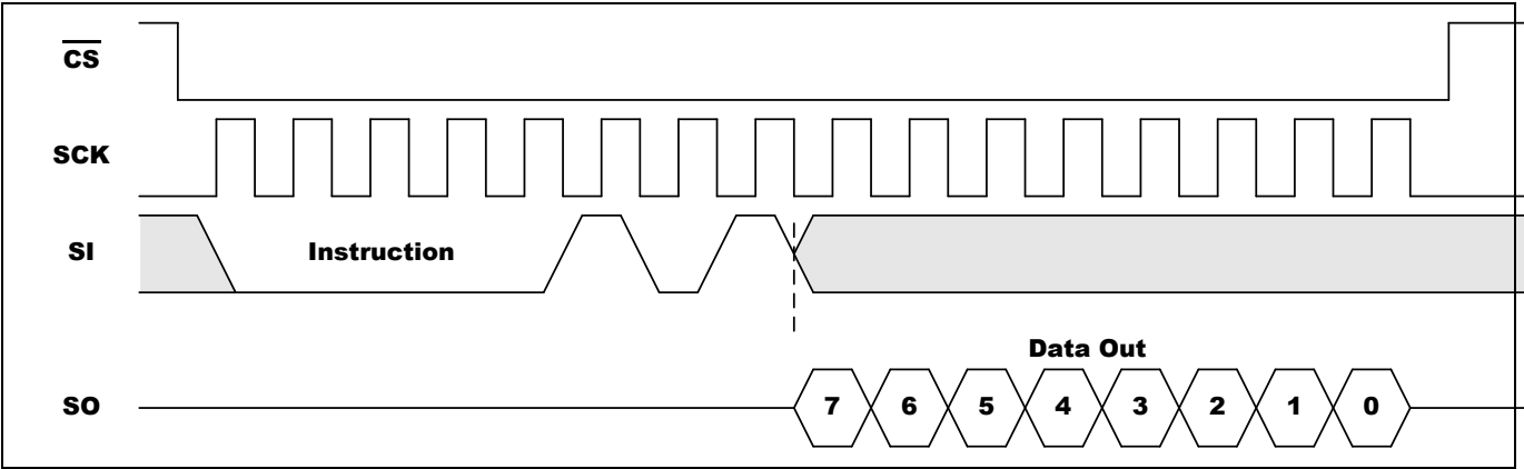
Figure 5-3. RDSR Sequence
