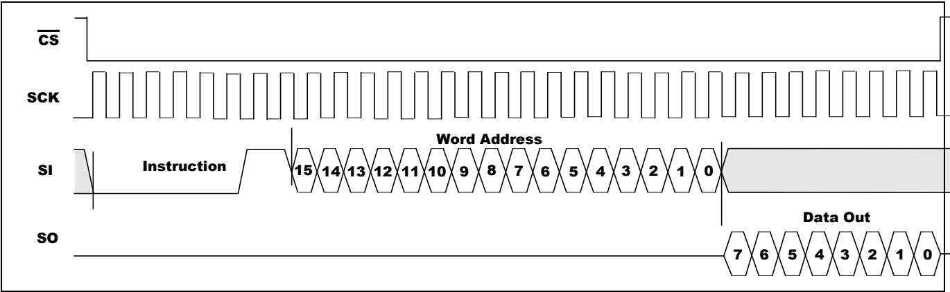
Figure 5-5. READ Sequence
