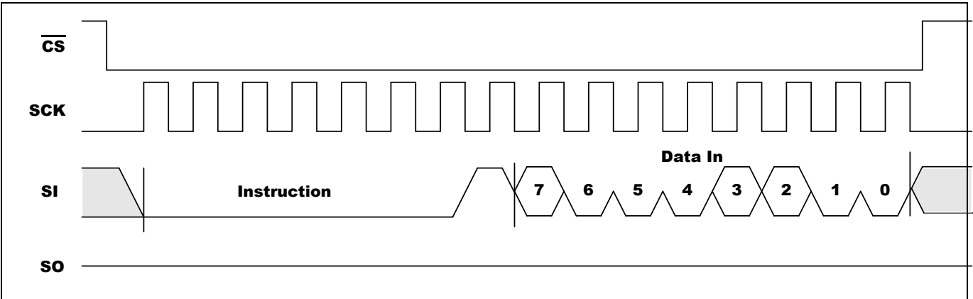
Figure 5-4. WRSR Sequence
