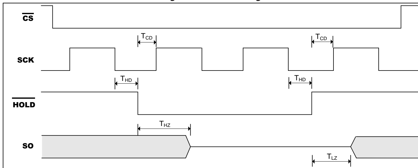
Figure 7-2. HOLD Timing
