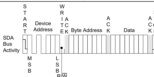
Figure 6. Byte Write
